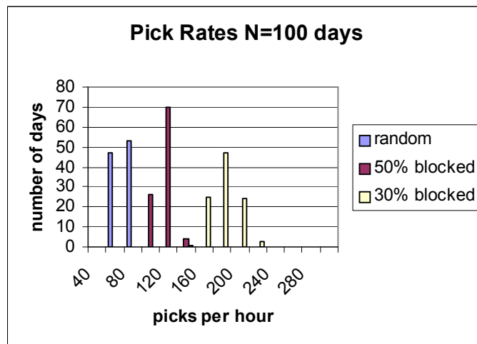
Figure 4: Simulated pick rates for 3 storage strategies
